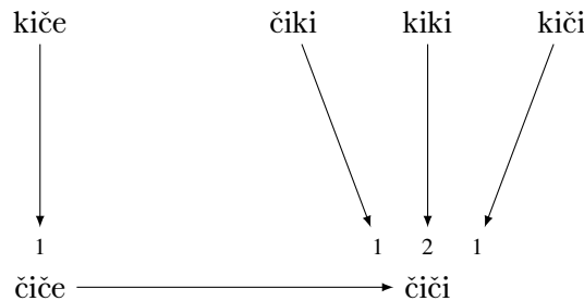
Figure 9: Output-rank increase
