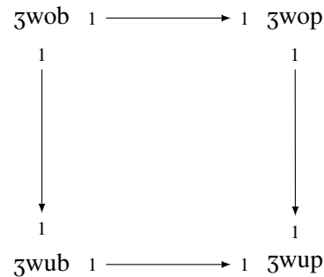
Figure 38: No interaction
